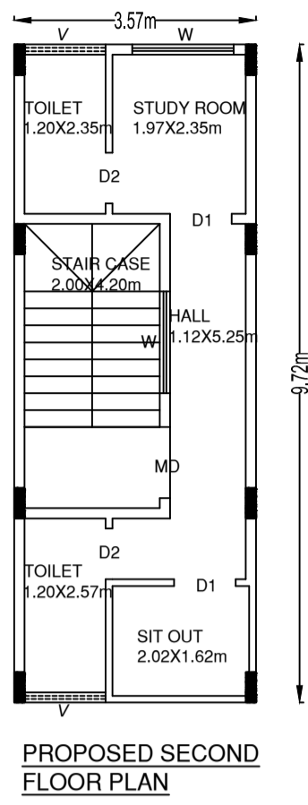
PROPOSED SECOND FLOOR PLAN
