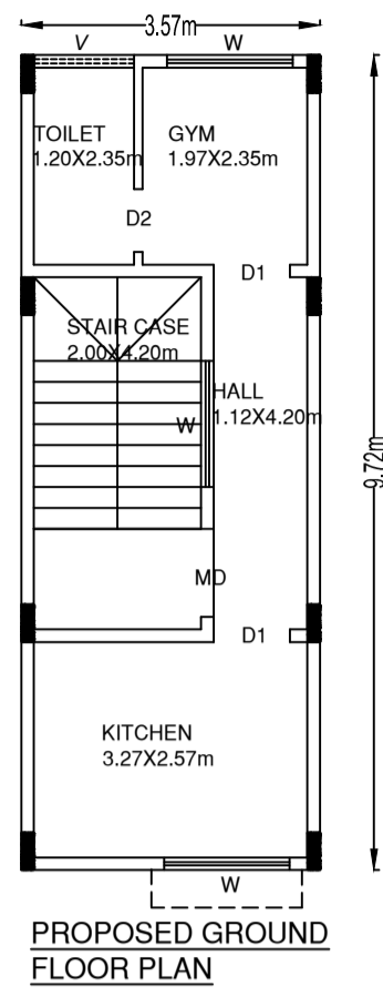
PROPOSED GROUND FLOOR PLAN
