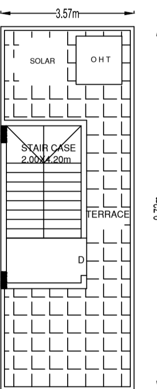
PROPOSED TERRACE FLOOR PLAN
